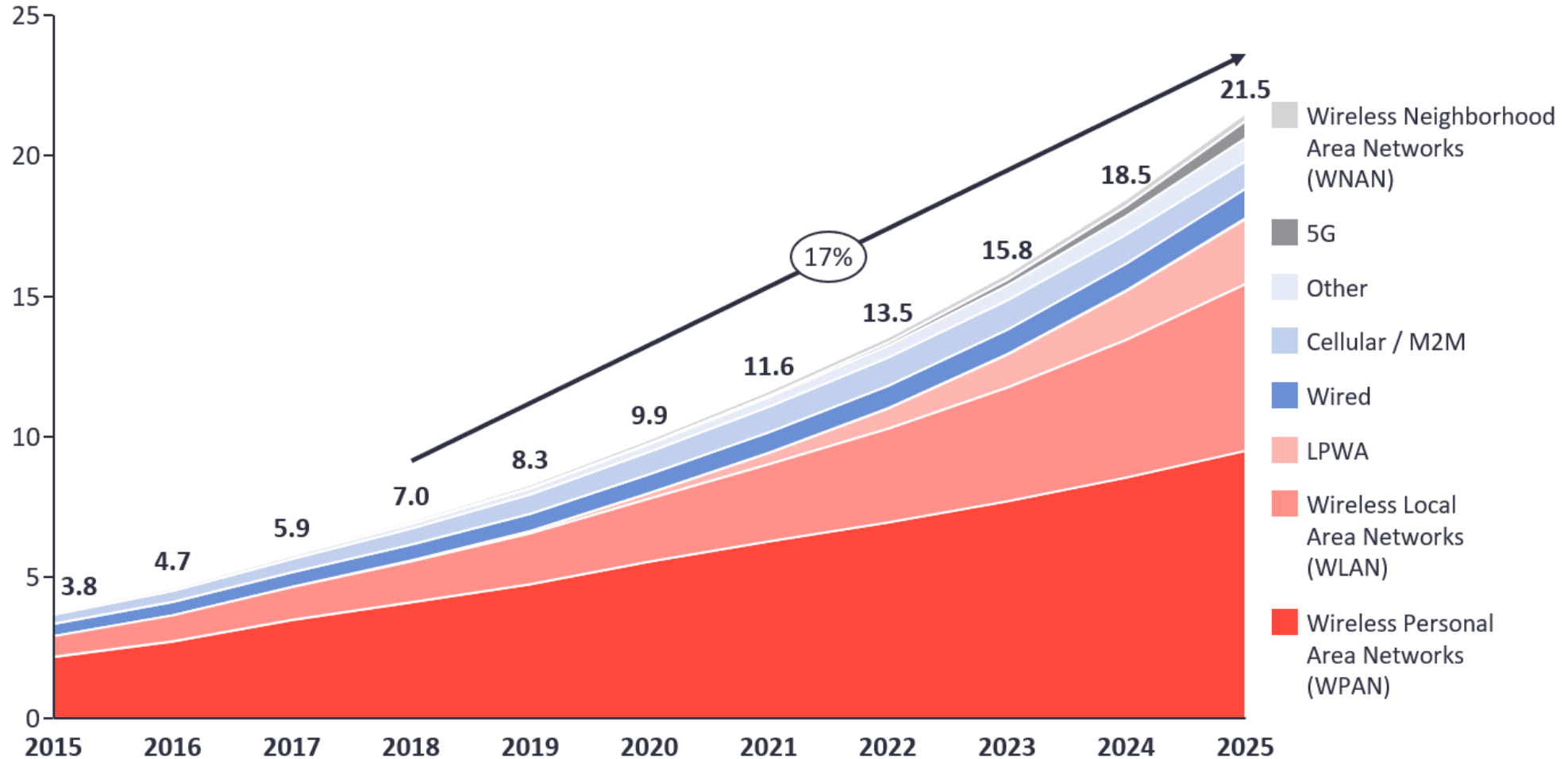
Number of global active IoT Connections (installed base) in Bn
